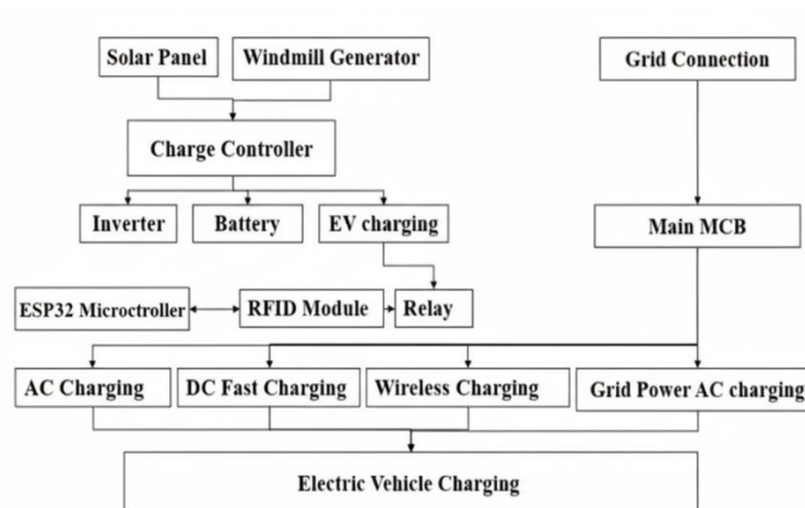
Fig. 1 Block Diagram of Proposed Project
