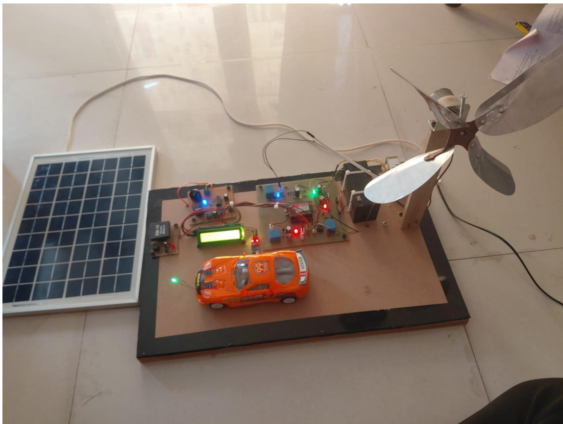
Fig. 2 Assembling and Testing of Components
